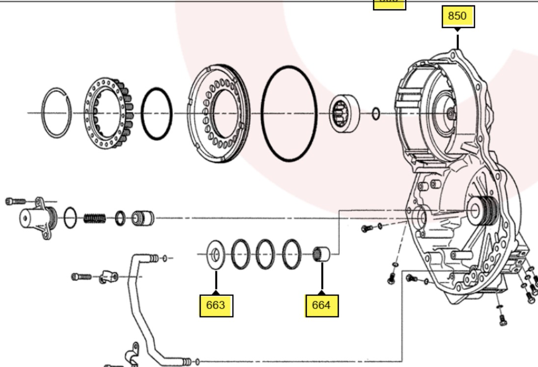
1 - 2 - Reverse Clutch Assy ('B5')
