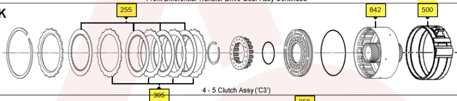
Front Differential Transfer Drive Gear Assy Continued
