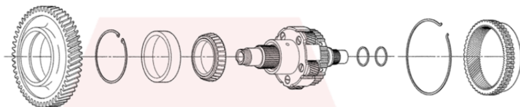
Front Differential Transfer Drive Gear Assy Continued
