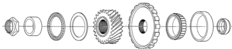
Front Differential Transfer Drive Gear Assy
