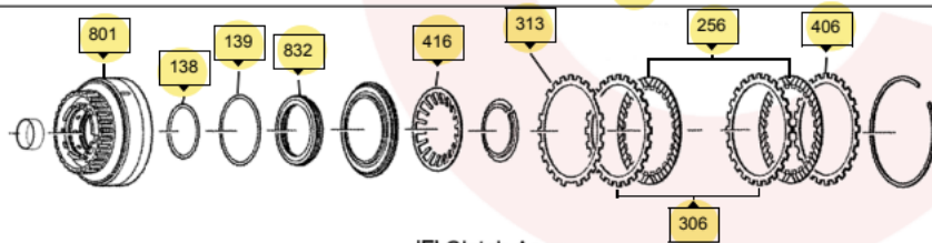
'F' Clutch Assy
