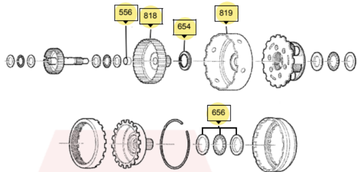
Front Planetary Assy
