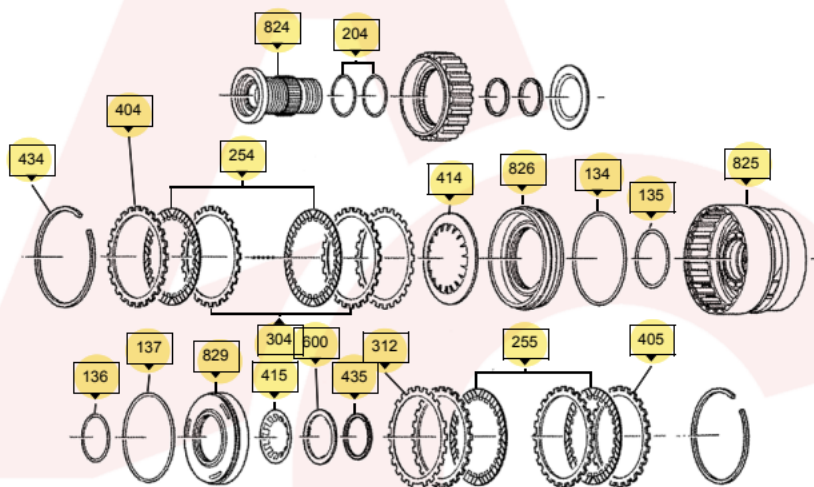
'D' &amp; 'G' Brake Assy
