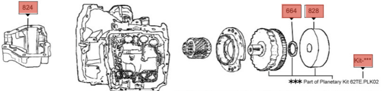
Pinion Gear, Output Shaft & Underdrive Ring Gear
