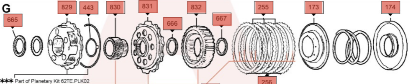
Planetary, Sun Gear & Hub
