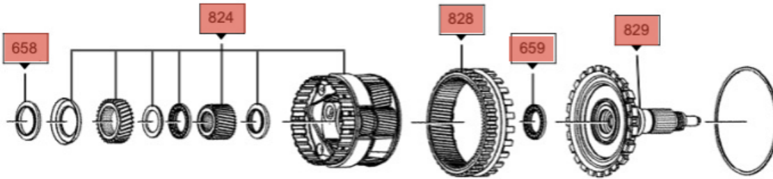
Rear Planetary Assembly
