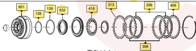
'F' Clutch Assy
