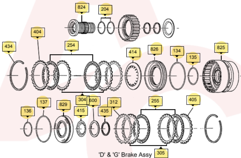
'D' &amp; 'G' Brake Assy
