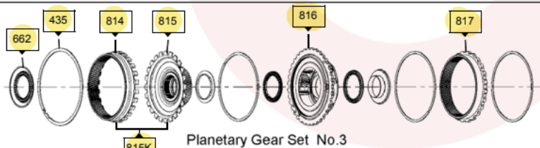
Planetary Gear Set No. 3
