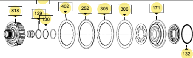
'E' Clutch
