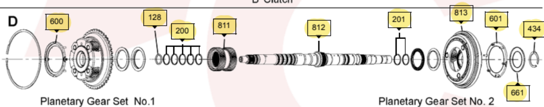
Planetary Gear Set No. 1
