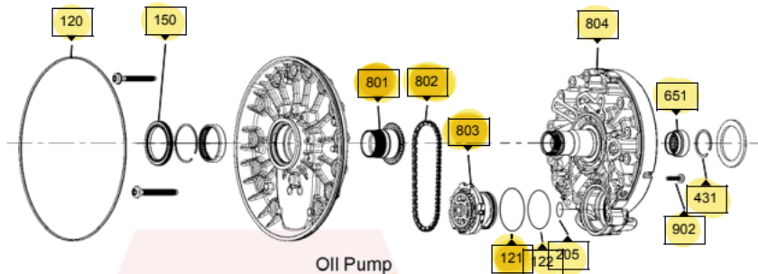
Oil Pump
