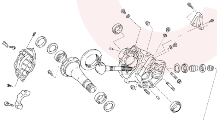
Casings, Differential, Counter Shaft and Valve Body Etc.
