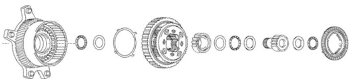
Counter Shaft Drive Gear, Rear Planetary &amp; Sun Gears
