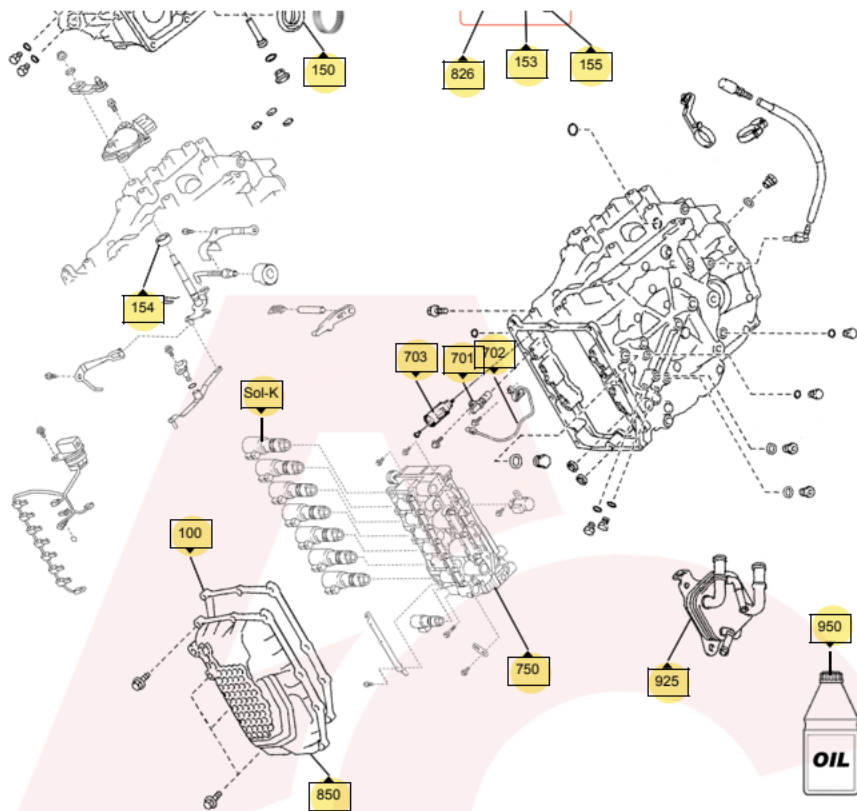
Casings, Differential, Counter Shaft and Valve Body Etc.
