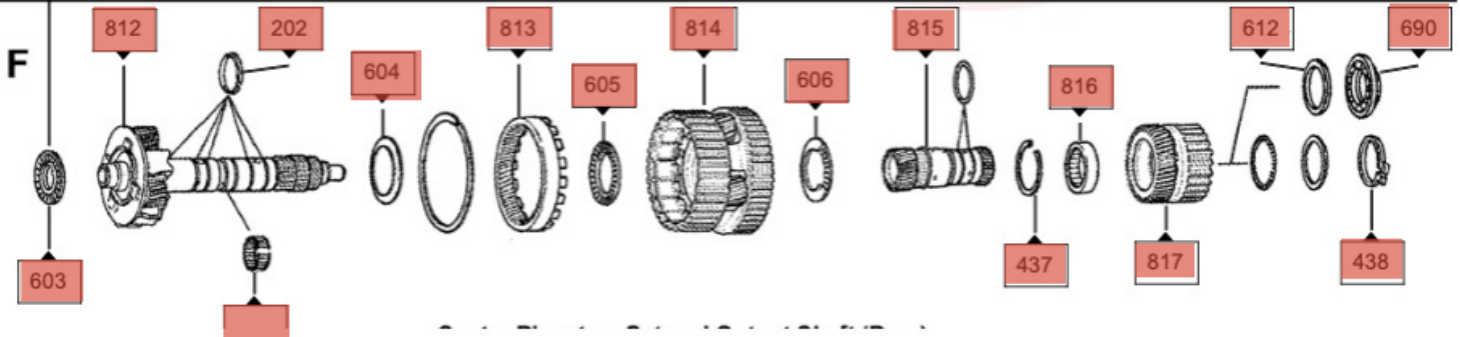
K2 Clutch
