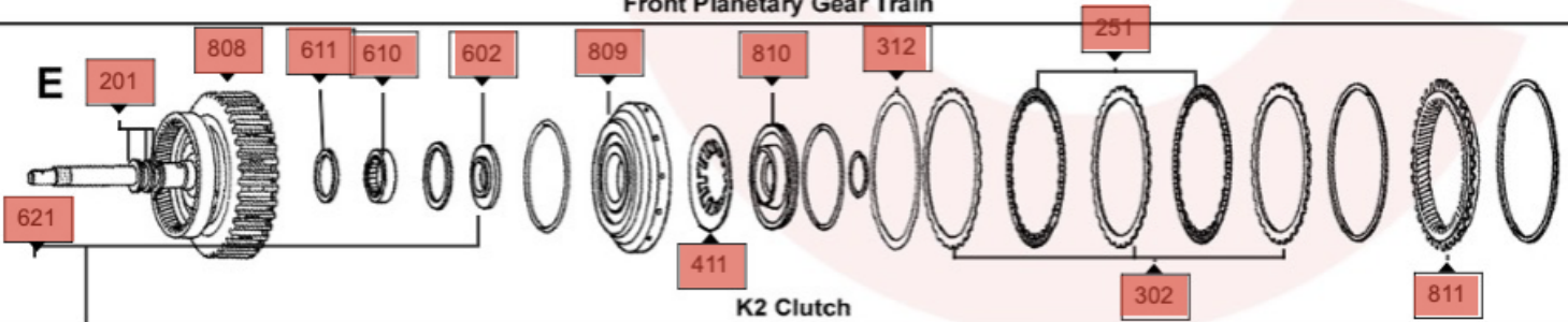
Front Planetary Gear Train
