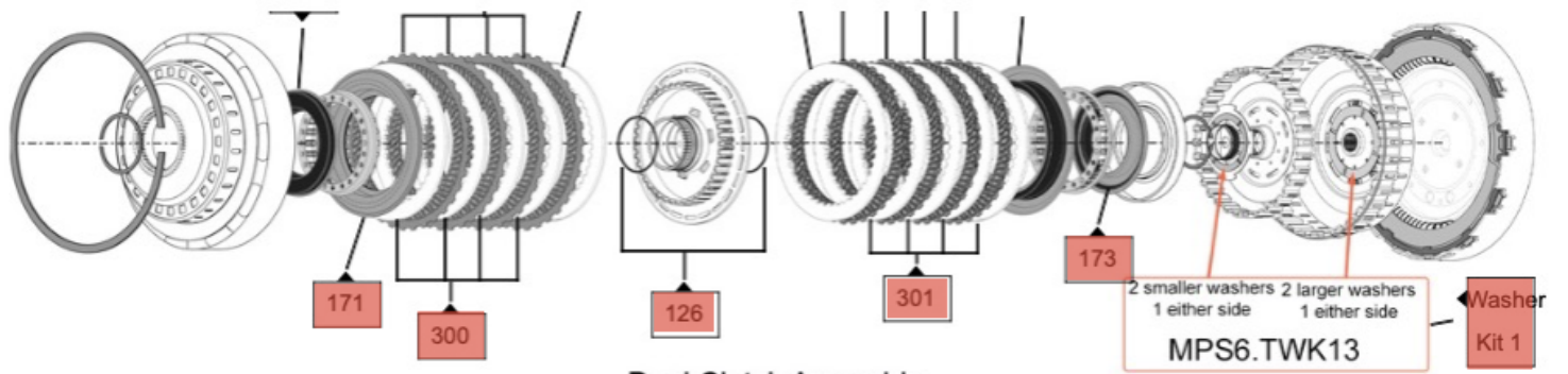
Dual Clutch Assembly
