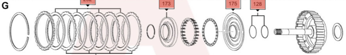
'C2' Clutch Assembly
