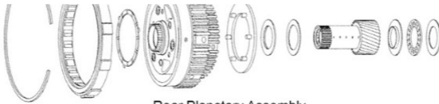
Rear Planetary Assembly
