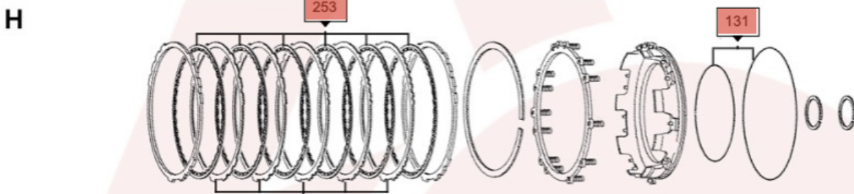
'B2' Brake Assembly
